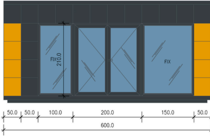
FRONT WALL
