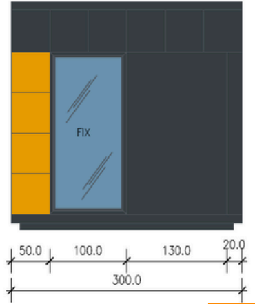
RIGHT WALL
